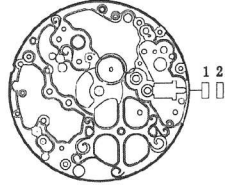
TY3600-2B (3600K) 17 Jewels
